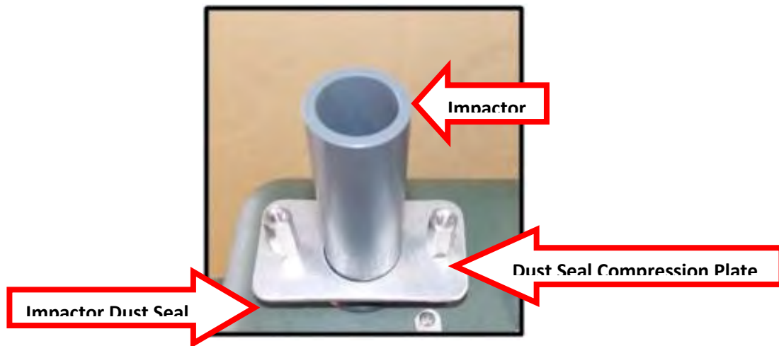
HAZ-SCANNER Dust Seal Compression Plate
