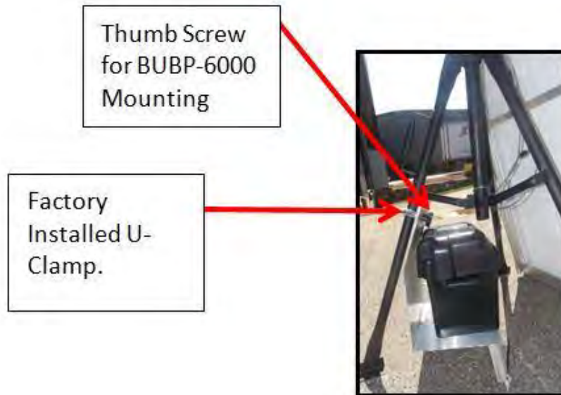
Back-up Battery Bracket Mounted on Tripod
