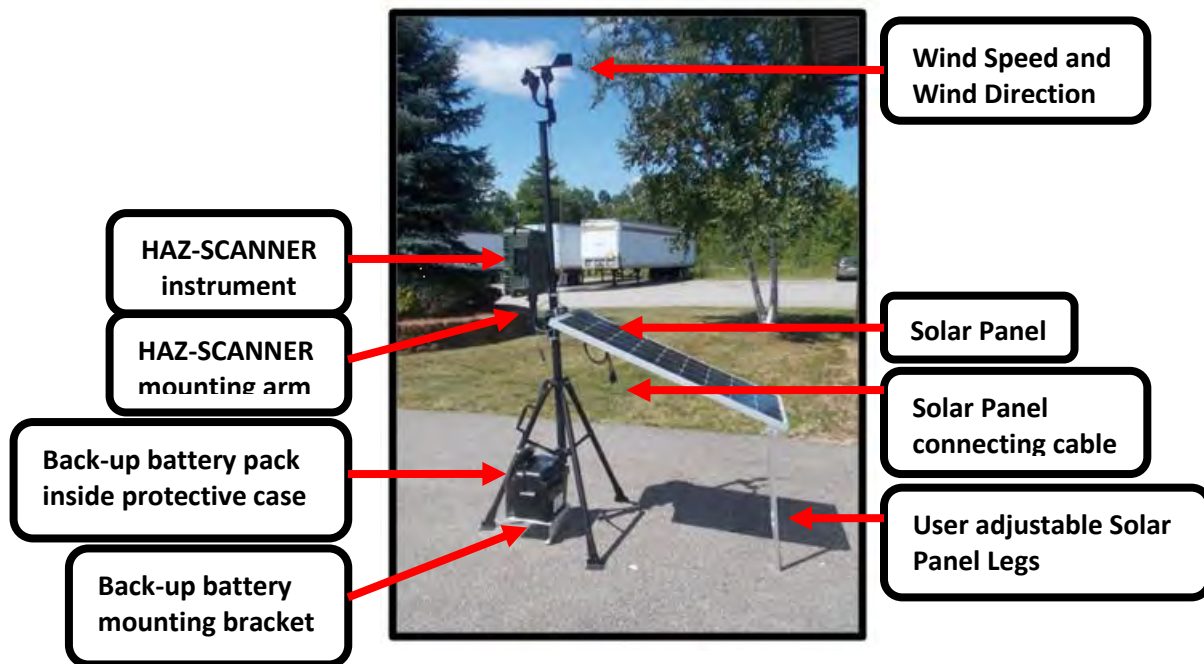
HAZ-SCANNER System – Tripod Mounting
