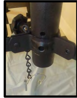
Raise mast until mast hole is above leg bracket
