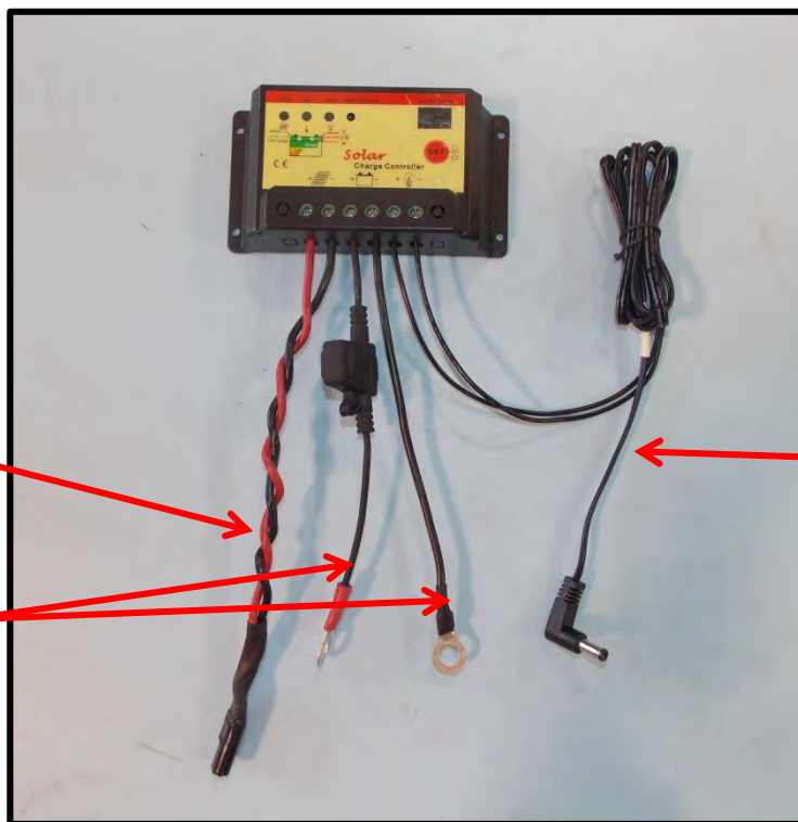
Solar Power Connections for Radio Repeater Configurations
