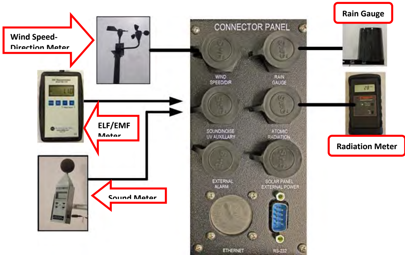
HAZ-SCANNER Peripheral Connections
